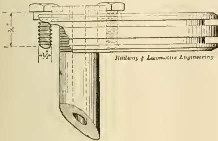
REVERSING PLATE BOLTS.
